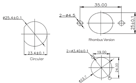
Panel Cut-Out(Circular & Square & Rhombus Version)
